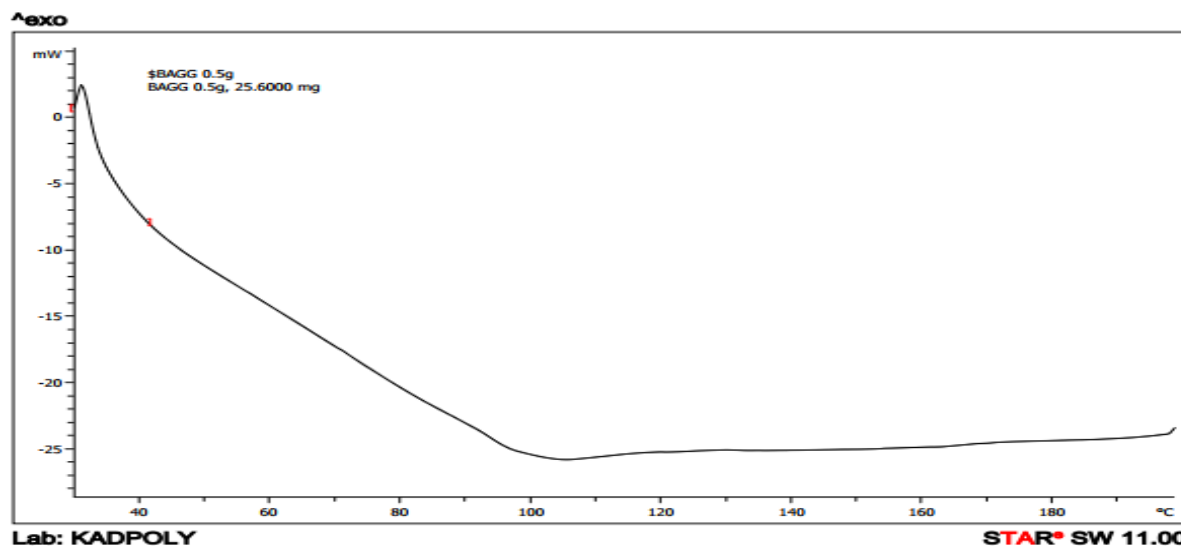
Figure 2: DSC Thermogram of BAGG
